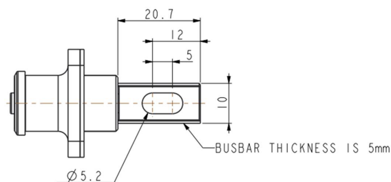
Busbar Termination
